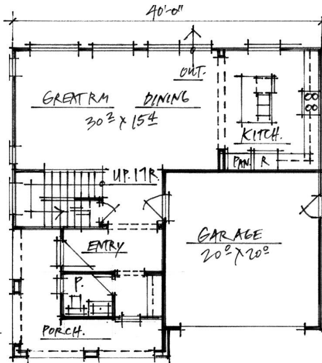
Side Entry 1st Flr. 945 sq. ft. 2nd Flr. 1,423 sq. ft. Total 2,368 sq. ft.
