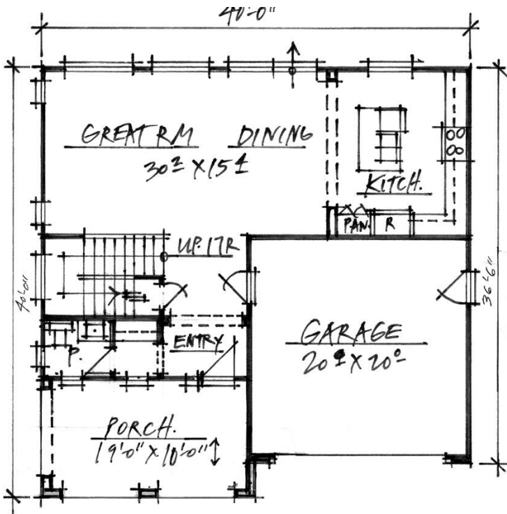
Maple Street Entry 1st Flr. 895 sq. ft. 2nd Flr. 1,423 sq. ft. Total 2,318 sq. ft.
