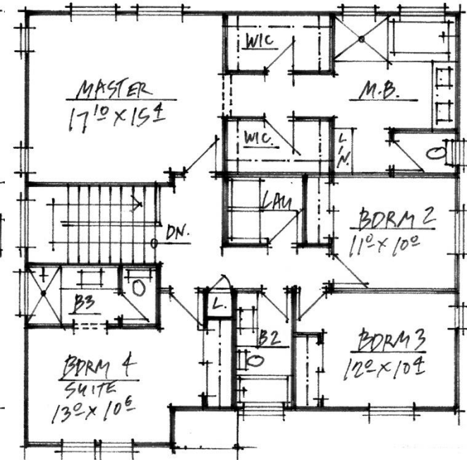
2nd flr. same for both 1st flr. Plans 2nd Flr. 1,423 sq. ft.
