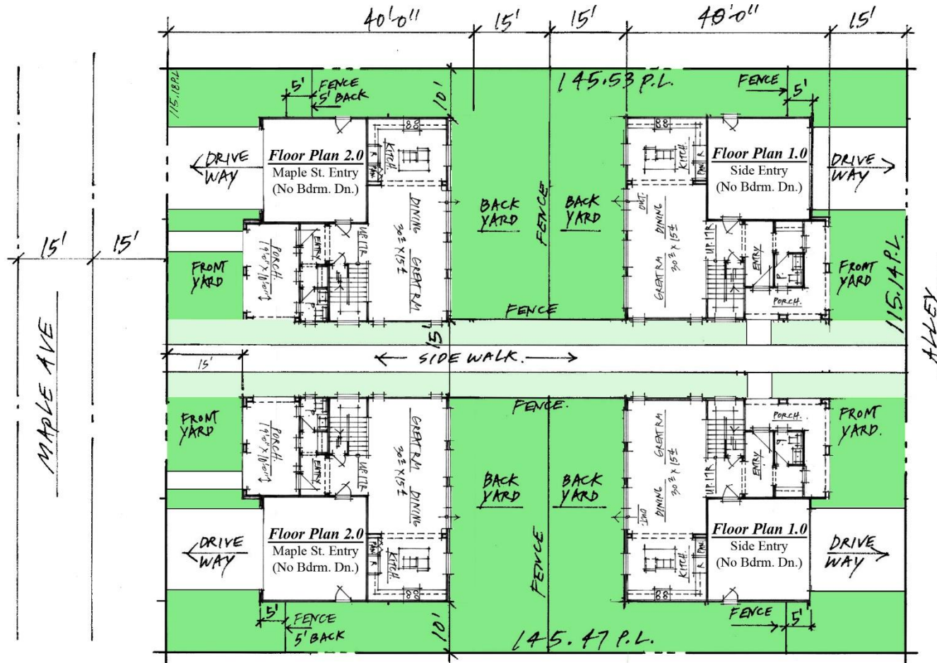
Conceptual Typical Plot with Plans 1.0 and 2.0 (a total of 2 floor plans) Maple Street Infill
